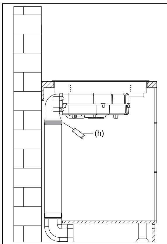
11. Secure both parts with the adhesive tape.
