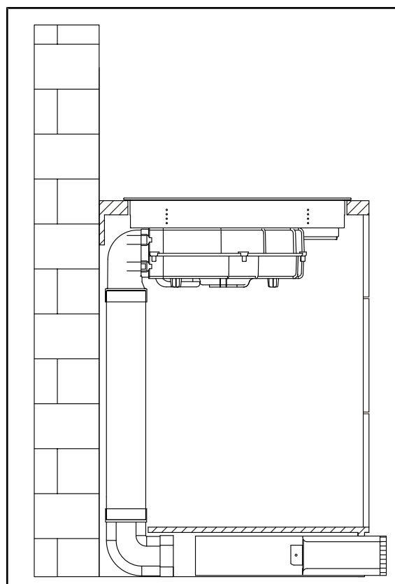
13. Install the recirculation cabinet adapter under the built-in cabinet.
